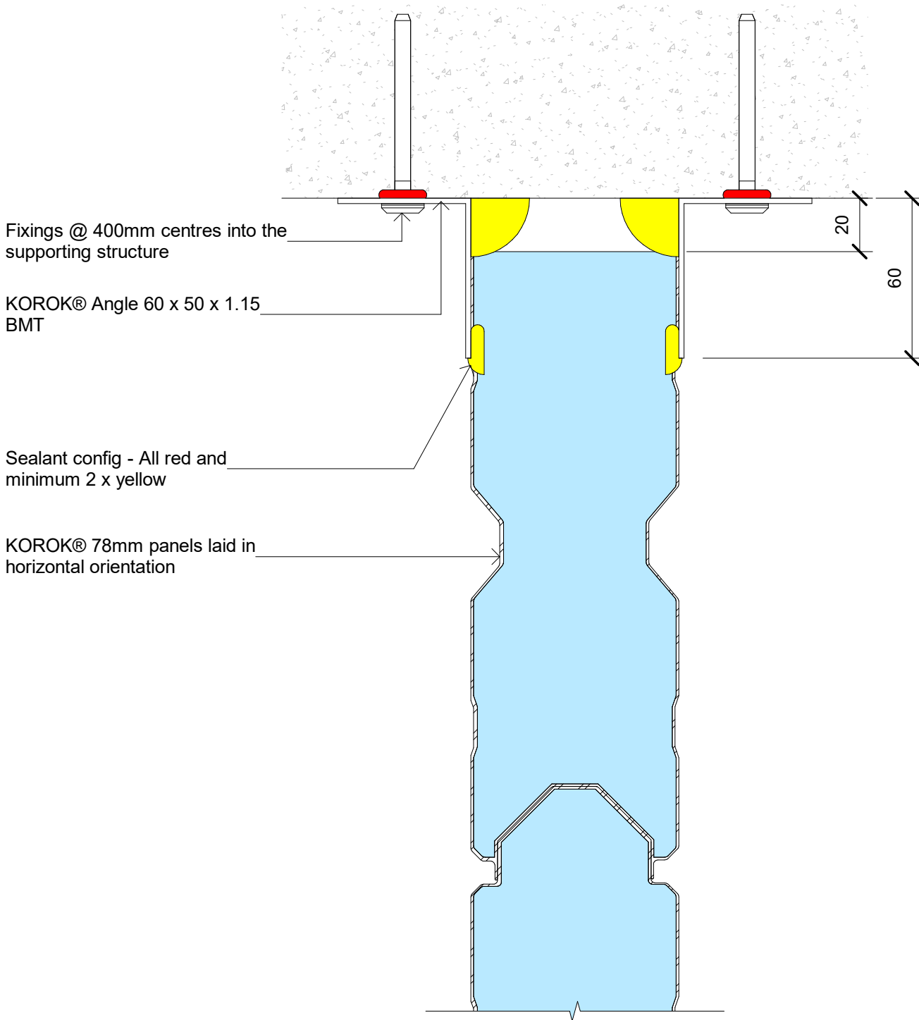
KOROK® 78m panel deflection head detail horizontal unsupported panel spans of up to 5000mm wide and unlimited wall height
