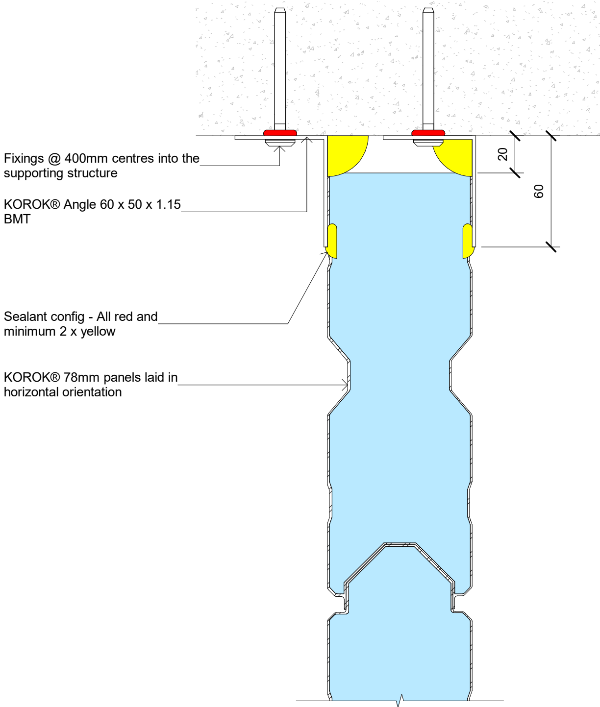
KOROK® 78m panel deflection head detail horizontal unsupported panel spans of up to 5000mm wide and unlimited wall height
